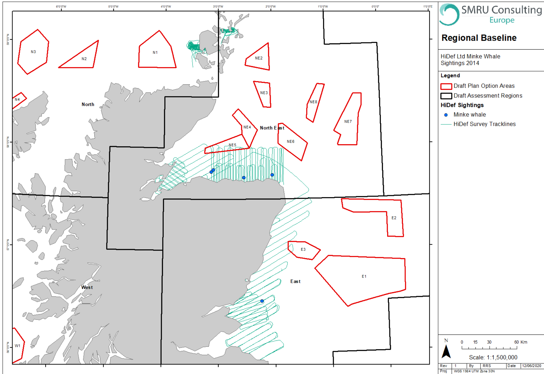
Figure 124: Minke whale sightings (blue dots) recorded during HiDef Ltd aerial surveys carried out in 2014.
