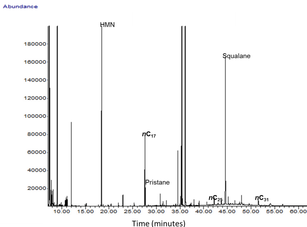
Figure 2: Aliphatic hydrocarbon profile of a mussel sample from a Loch Roag shellfish farm. Heptamethylnonane (HMN) and squalane were used as internal standards.
