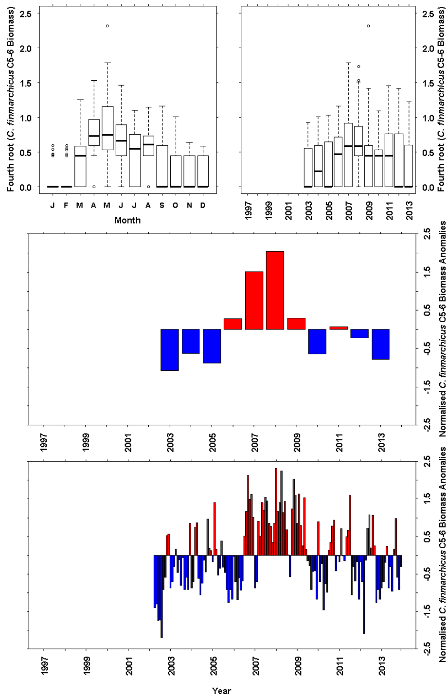
Figure 12.3 Calanus finmarchicus Stages C5-6 Biomass ( \text{mg dry weight m}^{-3} ) data from the long term monitoring site at Loch Ewe. a) Monthly boxplot of C. finmarchicus stages C5-6 biomass data. b) Annual boxplot of C. finmarchicus stages C5-6 biomass data. c) Annual mean anomaly time series d) Monthly mean anomaly time series. Sampling began in April 2002. Figures b and d only include data from January 2003. The full dataset was used as the base period for the anomaly calculations.
