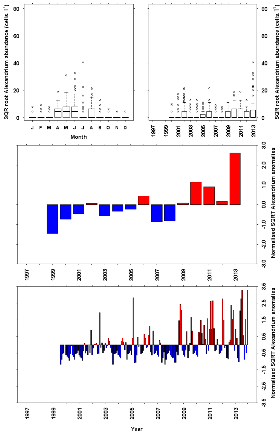
Figure 9.15 Alexandrium abundance (cells L -1 ) from the long term monitoring site at Loch Ewe. SQRT transformed data has been plotted. a) Monthly boxplot of Alexandrium abundance. b) Annual boxplot of Alexandrium abundance. c) Annual mean anomaly time series d) Monthly mean anomaly time series. Sampling for harmful species began in 1998. The full dataset was used as the base period for the anomaly calculations.
