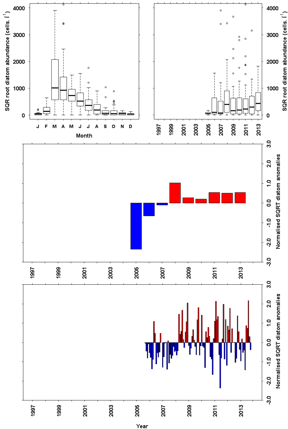
Figure 9.1 Diatom abundance (cells L^{-1} ) from the long term monitoring site at Millport. SQRT transformed data has been plotted. a) Monthly boxplot of diatom abundance. b) Annual boxplot of diatom abundance. c) Annual mean anomaly time series d) Monthly mean anomaly time series. Sampling began in October 2005 and finished in October 2013. The full dataset was used as the base period for the anomaly calculations.
