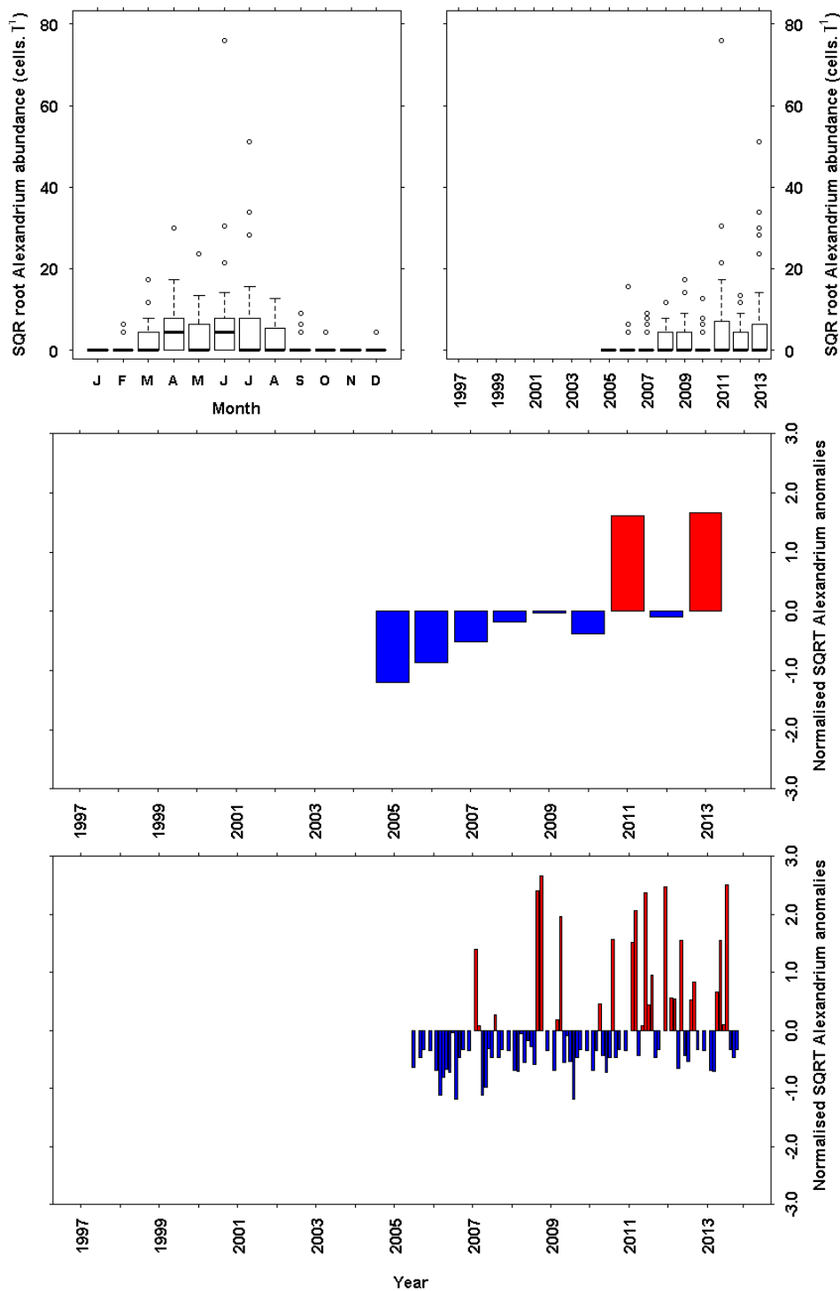
Figure 9.13 Alexandrium abundance (cells L -1 ) from the long term monitoring site at Millport. SQR T transformed data has been plotted. a) Monthly boxplot of Alexandrium abundance. b) Annual boxplot of Alexandrium abundance. c) Annual mean anomaly time series d) Monthly mean anomaly time series. Sampling began in 2005. The full dataset was used as the base period for the anomaly calculations.
