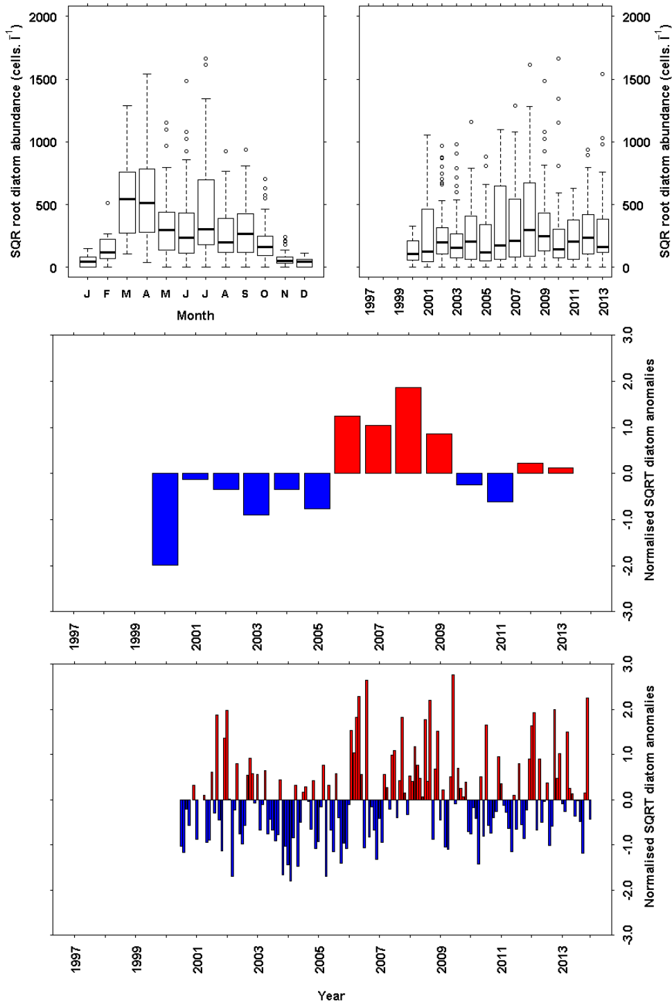
Figure 9.4 Diatom abundance (cells L^{-1} ) from the long term monitoring site at Scapa. SQR transformed data has been plotted. a) Monthly boxplot of diatom abundance. b) Annual boxplot of diatom abundance. c) Annual mean anomaly time series d) Monthly mean anomaly time series. Sampling began in 2001. The full dataset was used as the base period for the anomaly calculations.
