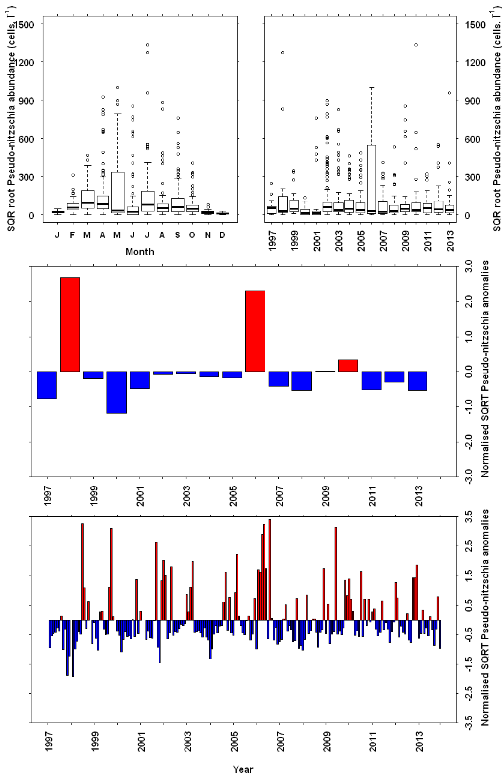
Figure 9.29 Pseudo-nitzschia abundance (cells L -1 ) from the long term monitoring site at Scapa. SQRT transformed data has been plotted. a) Monthly boxplot of Pseudo-nitzschia abundance. b) Annual boxplot of Pseudo-nitzschia abundance. c) Annual mean anomaly time series d) Monthly mean anomaly time series. Sampling for harmful species began in 1997. The full dataset was used as the base period for the anomaly calculations.
