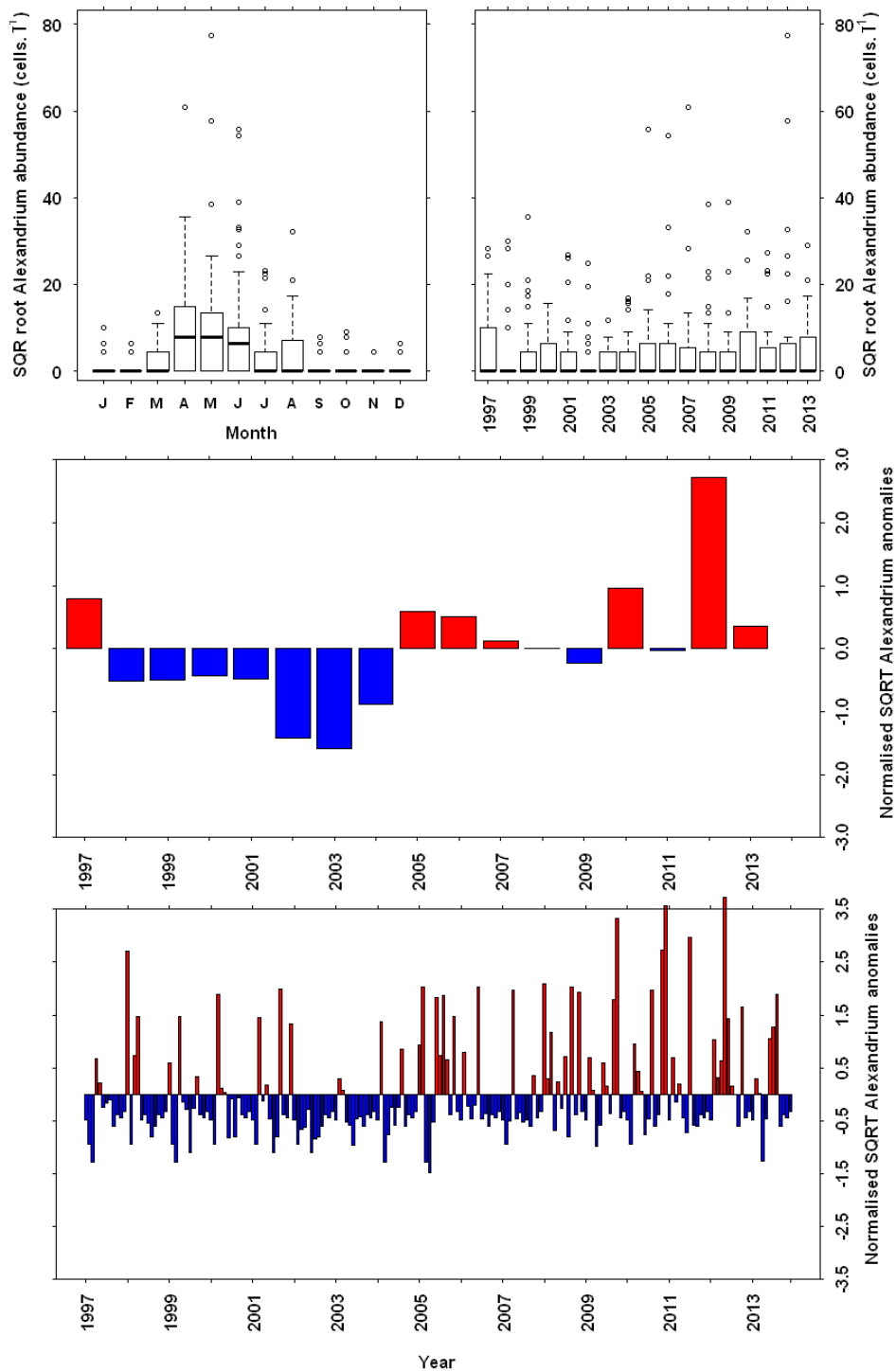
Figure 9.18 Alexandrium abundance (cells L -1 ) from the long term monitoring site at Stonehaven. SQR transformed data has been plotted. a) Monthly boxplot of Alexandrium abundance. b) Annual boxplot of Alexandrium abundance. c) Annual mean anomaly time series d) Monthly mean anomaly time series. Sampling for harmful species began in 1997. The full dataset was used as the base period for the anomaly calculations.
