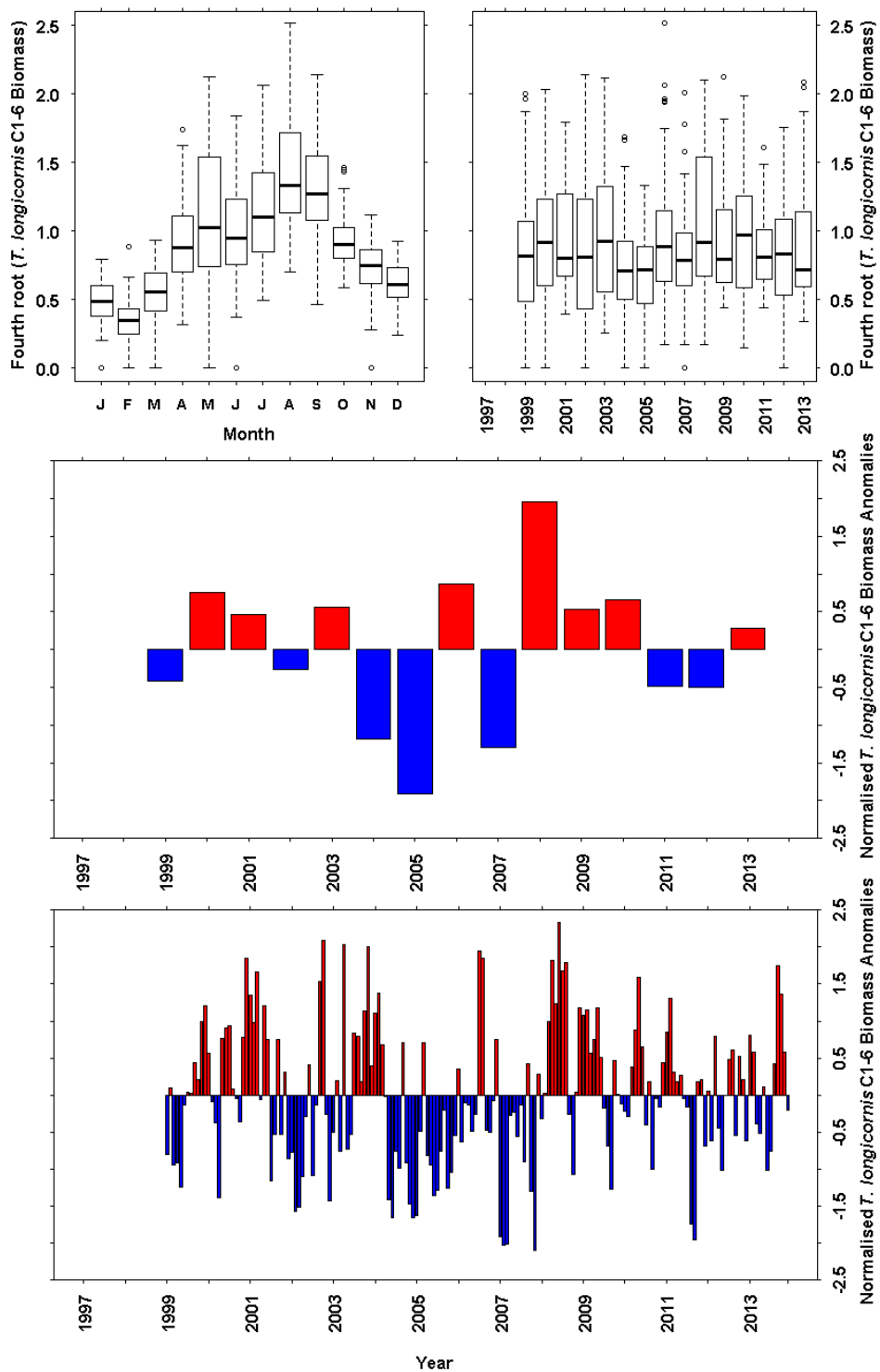
Figure 12.18 Temora longicornis Stages C1-6 Biomass ( \text{mg dry weight m}^{-3} ) data from the long term monitoring site at Stonehaven. a) Monthly boxplot of T. longicornis stages C1-6 biomass data. b) Annual boxplot of T. longicornis stages C1-6 biomass data. c) Annual mean anomaly time series d) Monthly mean anomaly time series. The full dataset was used as the base period for the anomaly calculations.
