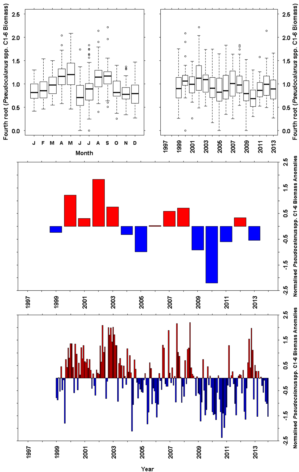
Figure 12.16 Pseudocalanus spp. Stages C1-6 Biomass (mg dry weight m -3 ) data from the long term monitoring site at Stonehaven. a) Monthly boxplot of Pseudocalanus spp. stages C1-6 biomass data. b) Annual boxplot of Pseudocalanus spp. stages C1-6 biomass data. c) Annual mean anomaly time series d) Monthly mean anomaly time series. The full dataset was used as the base period for the anomaly calculations.
