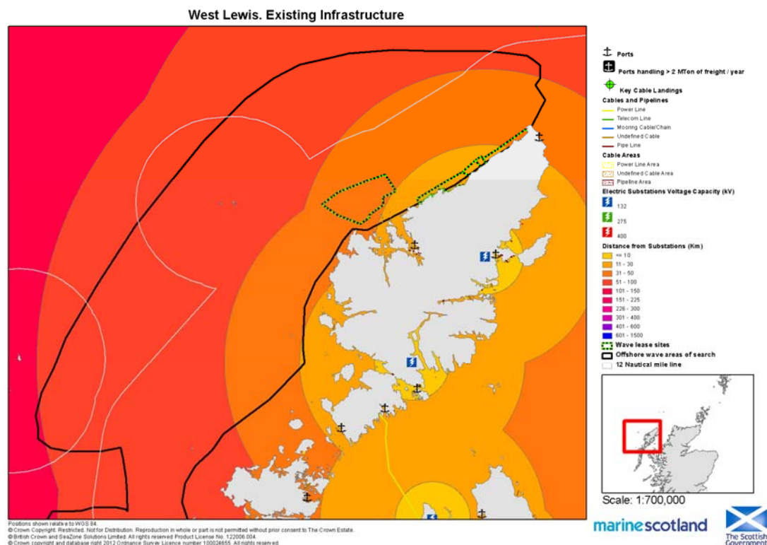
Fig.4.23 Existing Infrastructure in the West of Hebrides (West Lewis) (Area of Search)
